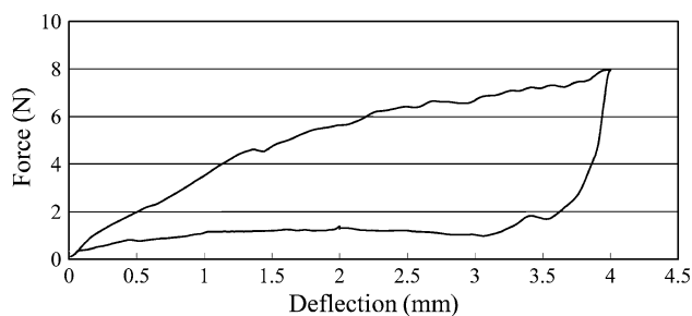
Fig. 11 TPB curve of solution treated and aged wire at 400^\circ C for 30 min
