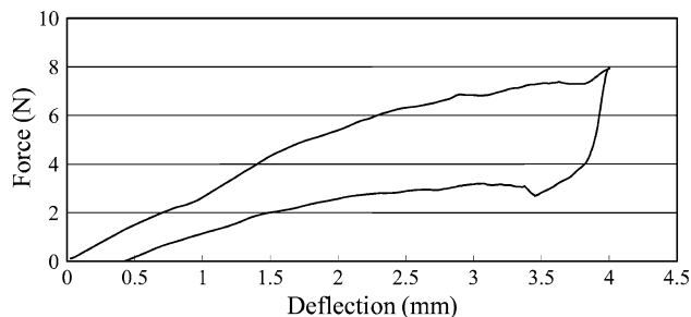
Fig. 12 TPB curve of solution treated and aged wire at 400^\circ C for 60 min
