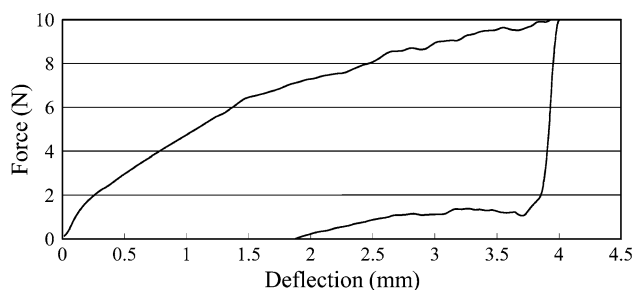
Fig. 10 TPB curve of solution treated and aged wire at 400^\circ C for 10 min
