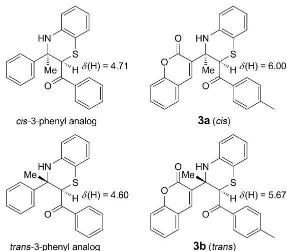
Fig. 1. The comparison of \text{H}-\text{C}(2) chemical shifts in cis - and trans -isomers. The selected ^1\text{H} -NMR data of 3-Ph analogs was reported by Mashraqui and Kellogg [6].
