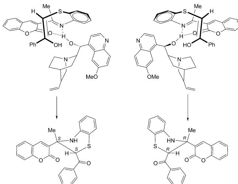
Fig. 5. cis -Diastereoselectivity in organocatalysis by quinine and the lack of enantioselectivity
