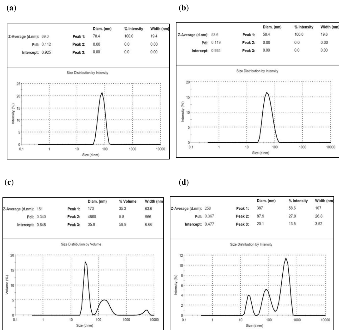
Fig. 1. Particle size of phenol-loaded NPs before being applied to the test culture (a: nano-ZnO and b: nano-TiO 2 ) and after 48 h in suspension (c: nano-ZnO and d: nano-TiO 2 ) of Malvern instrument DLS.
