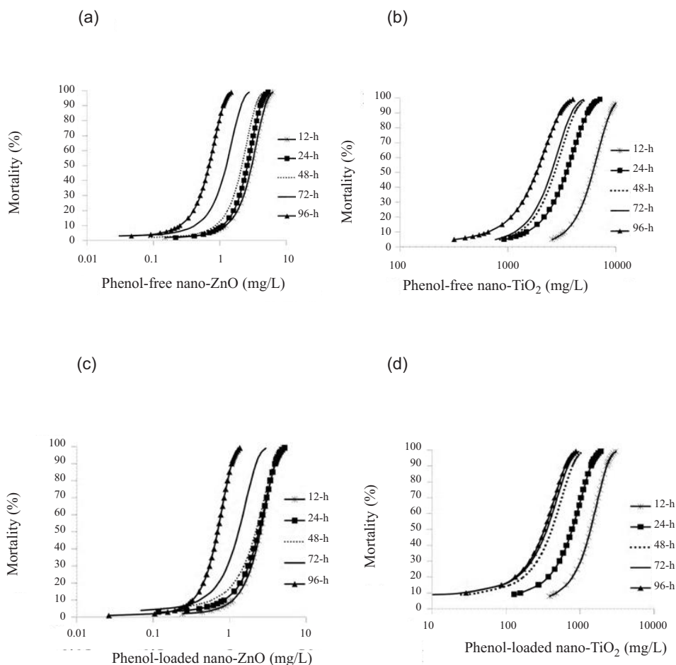
Fig. 2. Mortality rate for Daphnia magna at the various concentrations of phenol-free NPs (a and b) and phenol-loaded NPs (c and d) at different periods of time.
